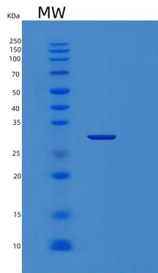
Figure 1. SDS-PAGE
