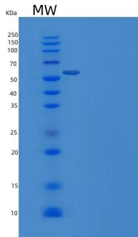
Figure 2. SDS-PAGE
