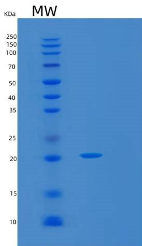
Figure 1. SDS-PAGE
