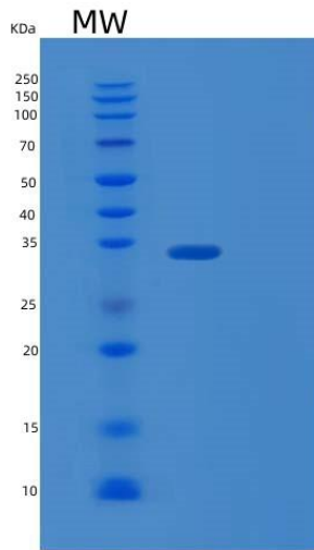
Figure . SDS-PAGE
