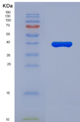
Figure 2. SDS-PAGE
