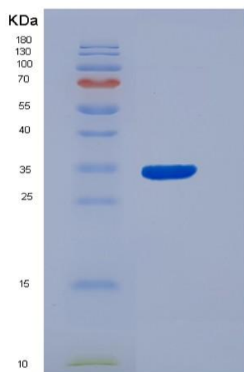
Figure . SDS-PAGE
