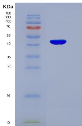
Figure . SDS-PAGE
