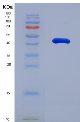
Figure 1. SDS-PAGE
