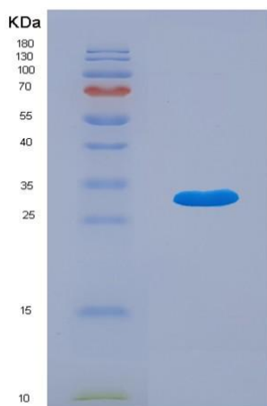
Figure . SDS-PAGE
