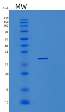
Figure . SDS-PAGE
