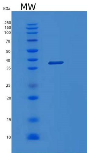
Figure 2. SDS-PAGE
