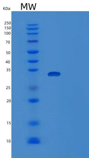
Figure 2. SDS-PAGE
