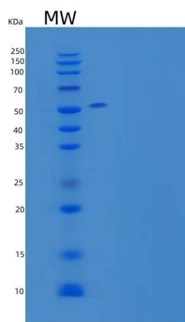
Figure 2. SDS-PAGE
