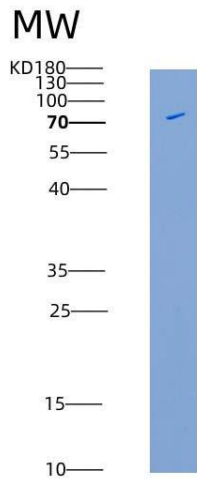
Figure . SDS-PAGE
