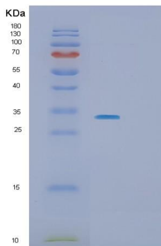
Figure 2. SDS-PAGE
