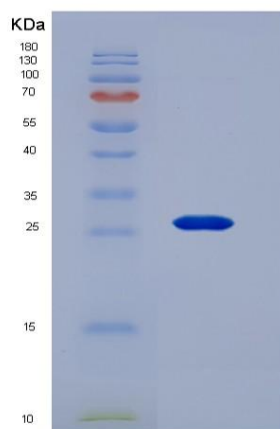
Figure . SDS-PAGE
