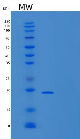
Figure . SDS-PAGE
