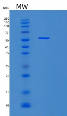
Figure . SDS-PAGE
