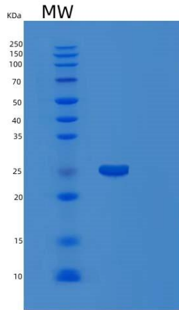
Figure 1. SDS-PAGE
