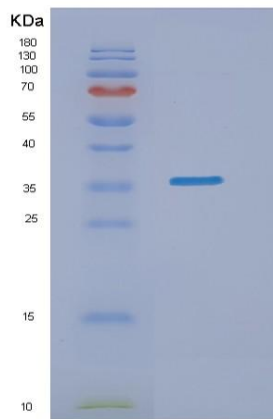
Figure . SDS-PAGE
