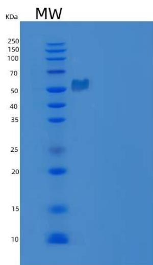
Figure . SDS-PAGE
