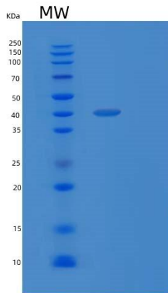
Figure 2. SDS-PAGE
