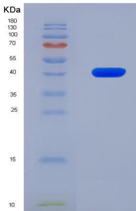
Figure 1. SDS-PAGE
