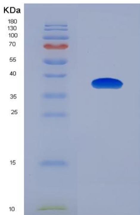
Figure . SDS-PAGE
