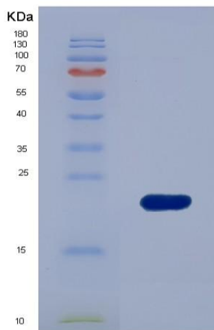
Figure . SDS-PAGE
