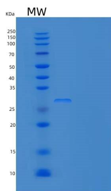
Figure . SDS-PAGE
