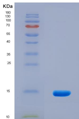
Figure . SDS-PAGE
