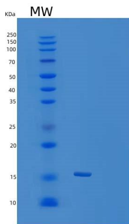
Figure . SDS-PAGE
