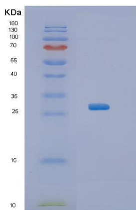
Figure 2. SDS-PAGE
