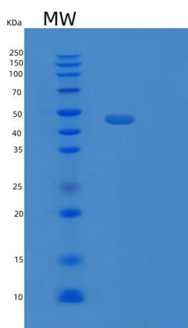
Figure . SDS-PAGE
