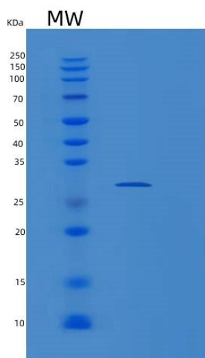
Figure 2. SDS-PAGE
