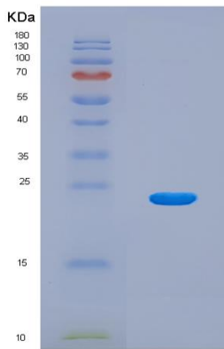
Figure 1. SDS-PAGE
