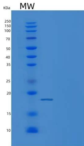
Figure . SDS-PAGE
