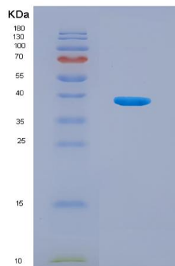
Figure . SDS-PAGE
