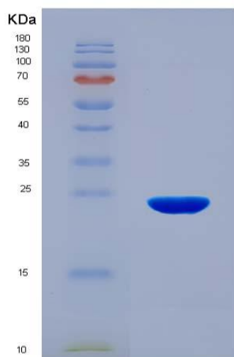
Figure . SDS-PAGE
