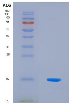
Figure 1. SDS-PAGE
