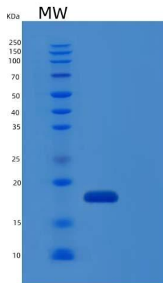
Figure 2. SDS-PAGE
