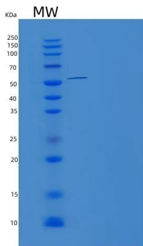
Figure . SDS-PAGE
