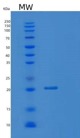
Figure . SDS-PAGE
