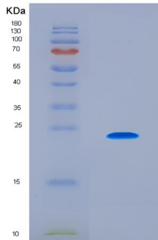
Figure 1. SDS-PAGE
