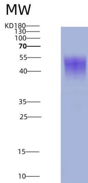
Figure 1. SDS-PAGE
