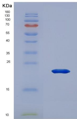
Figure 1. SDS-PAGE
