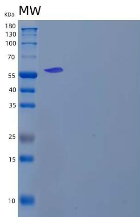
Figure . SDS-PAGE
