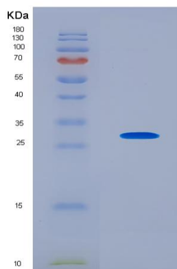
Figure 2. SDS-PAGE
