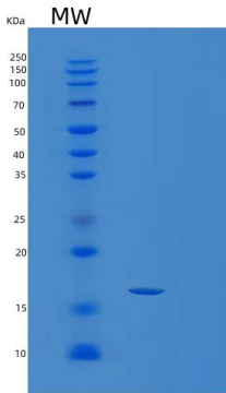
Figure 1. SDS-PAGE
