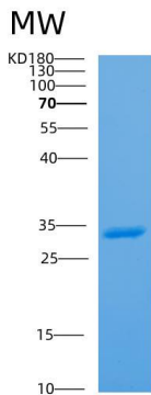
Figure 1. SDS-PAGE
