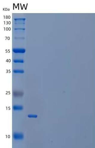
Figure . SDS-PAGE
