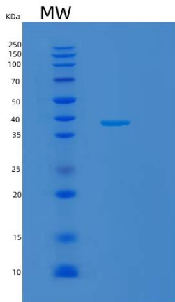
Figure 1. SDS-PAGE
