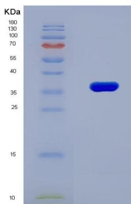
Figure 1. SDS-PAGE
