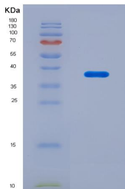
Figure 1. SDS-PAGE
